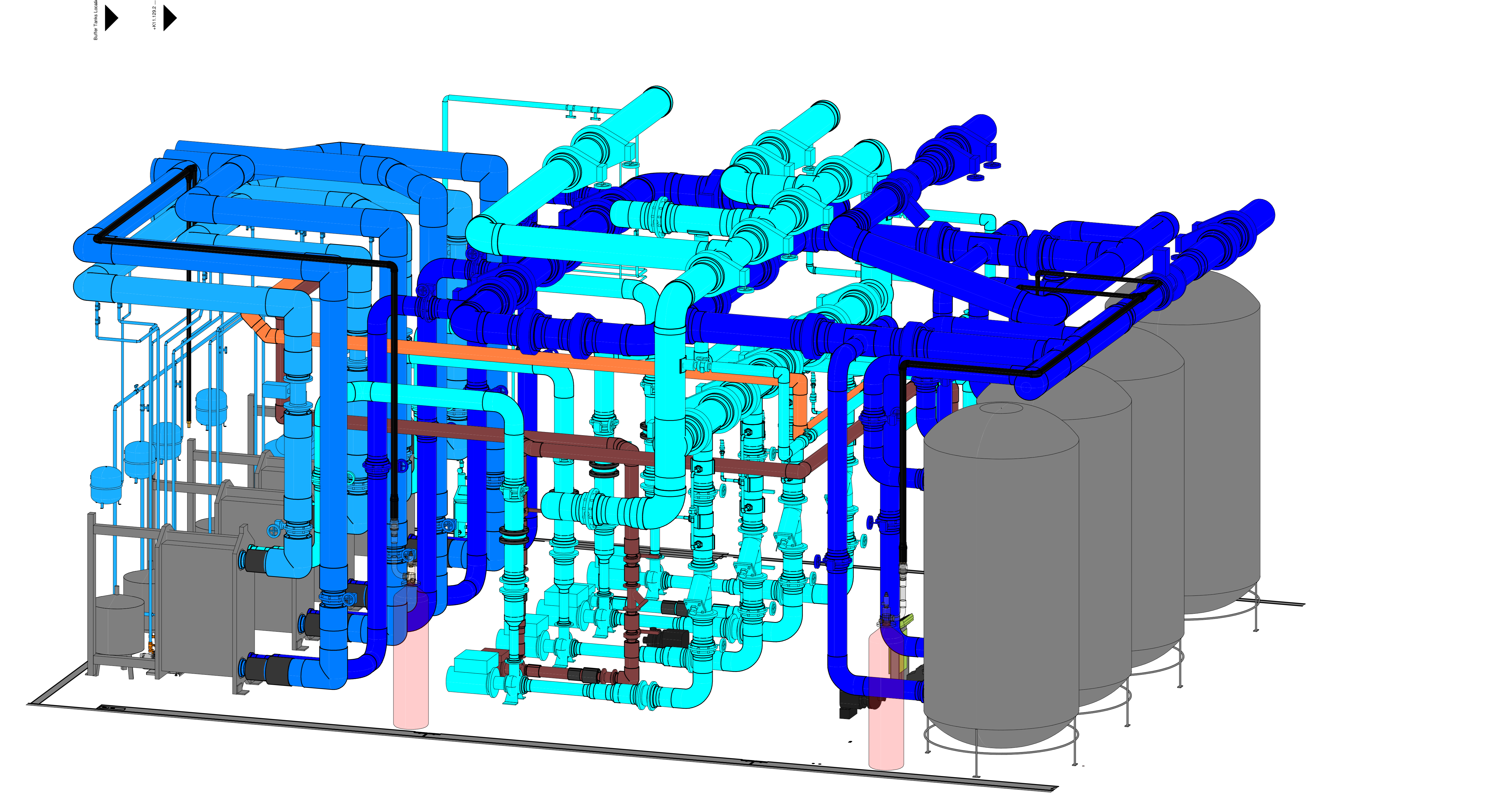
11.129 - 3D Room
